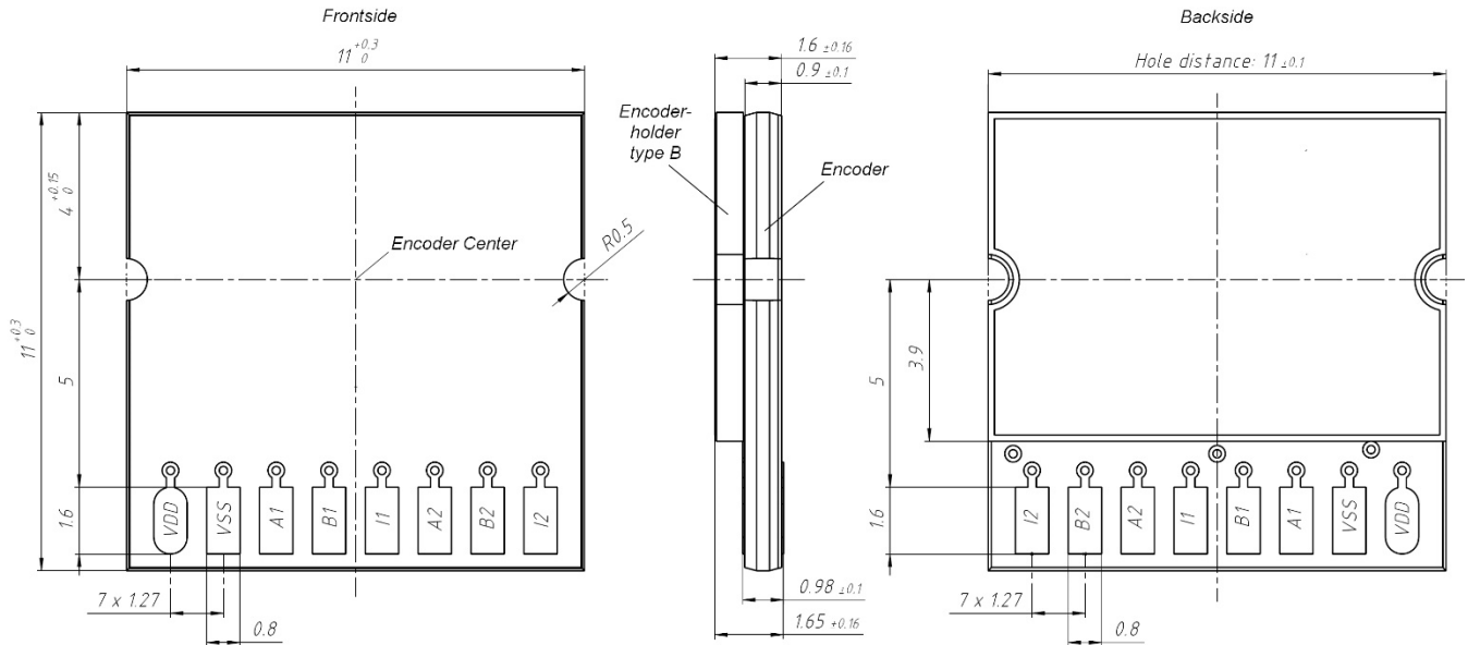
Fig. 3 Dimensions of IT3403 encoder on encoder-holder type B. The “Encoder center” must be centered with respect to the “Readout radius” of the Codewheel (Fig 4)
